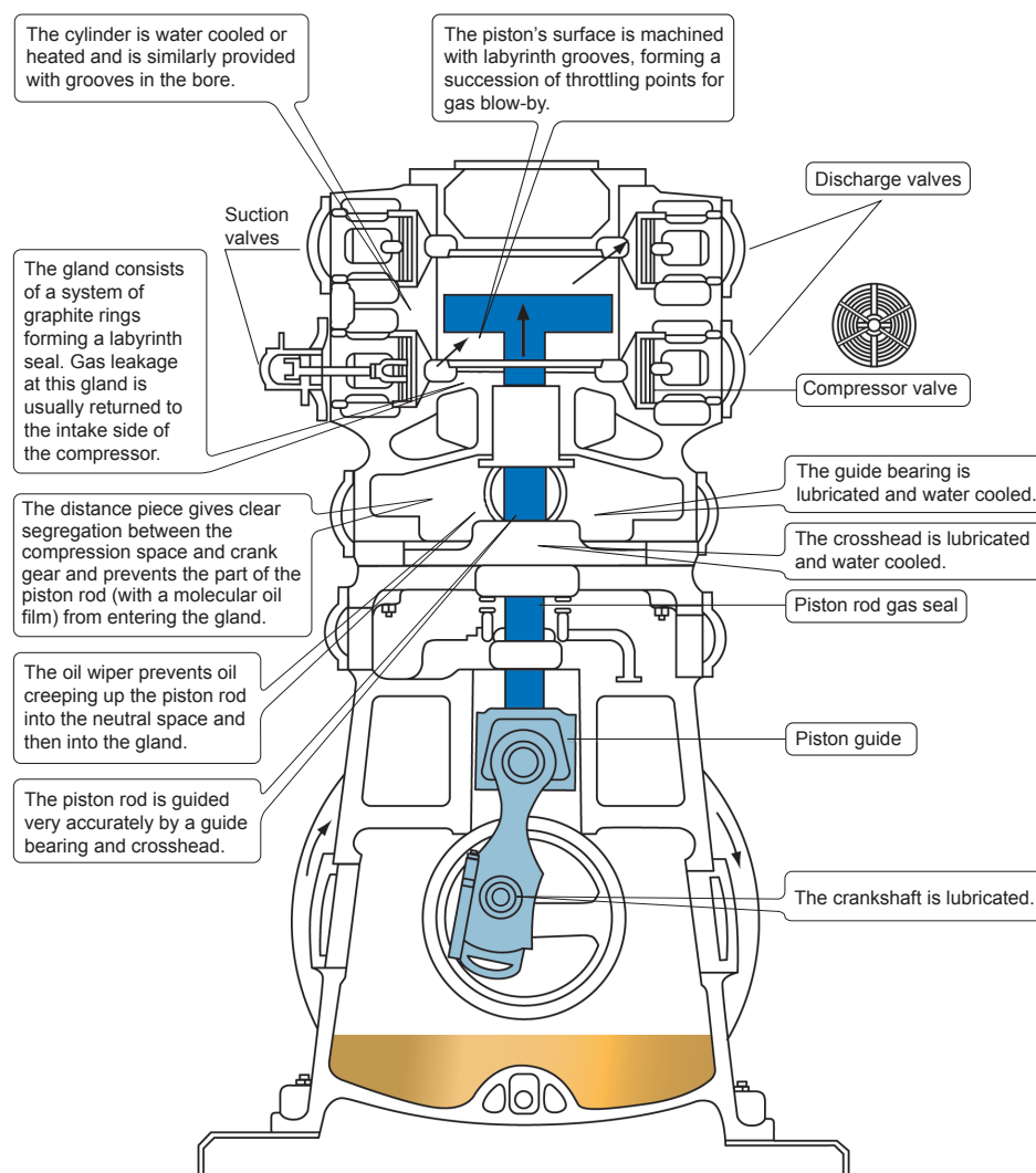
Figure 31.6: Oil-free compressor
