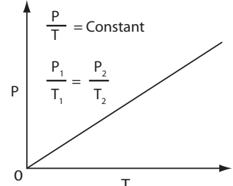
Figure 27.12(c): Pressure Law for gases (constant volume)
